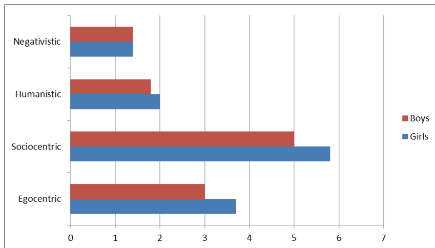
Fig. 3. The results of the diagnostic after I.D. Egorycheva's technique 'Personal orientation study'
