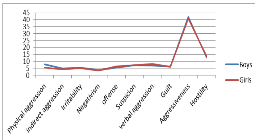
Fig. 1. The study results of the aggressiveness level diagnosis after the Bass-Perry questionnaire
