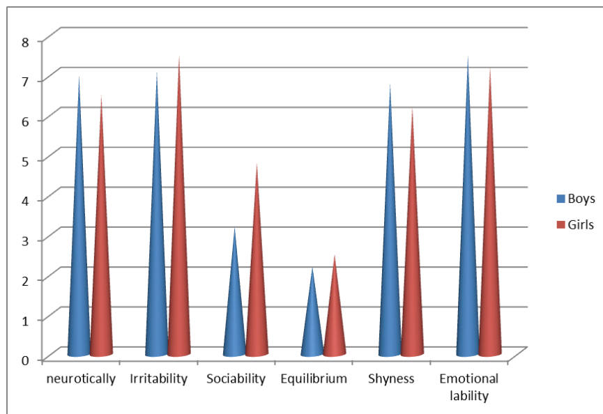
Fig. 2. The results of the diagnosis after using the modified Freiburg Personality Inventory/Form B (FPI-B)
