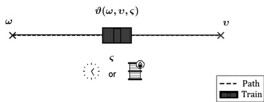
Figure 1. Example illustrating the degree of proximity between \omega and v with respect to \varsigma .
