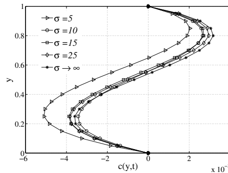
Fig. 7. Effect of \sigma on c(y, t) for \alpha = 0.5 , R = 0.5 , \omega t = \pi/4 , P_s = 1 , P_j = 1 , P_o = 1 , m = 0.5 , n = 0.5 .
