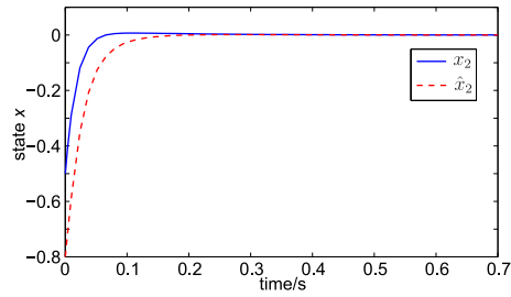
Fig. 7. Responses of states x_2, \hat{x}_2 .
