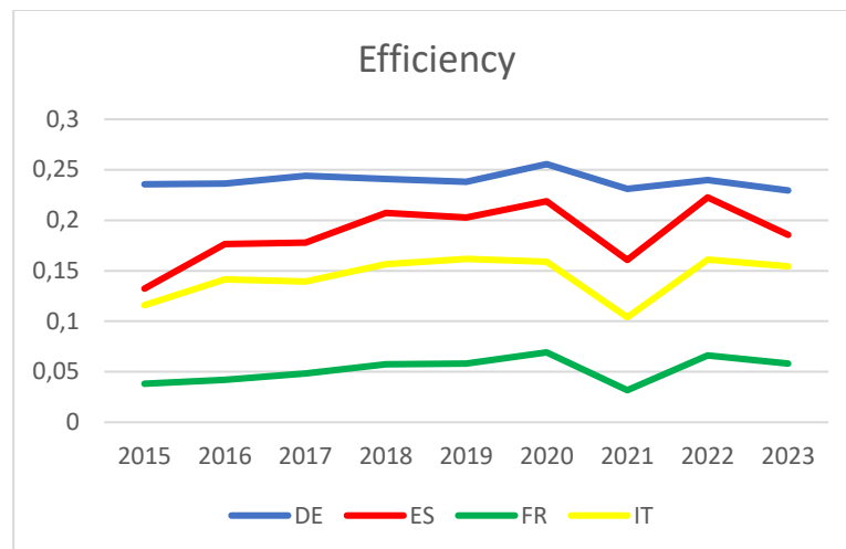
Figure 6. Efficiency for Each DMU in the Reference Set for the Simplified Efficiency Model by Country
