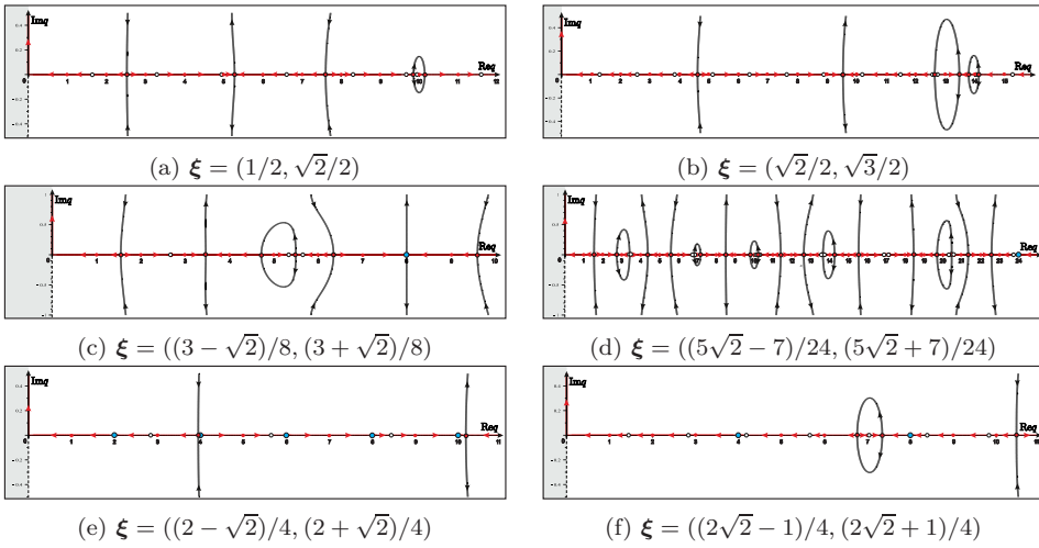
Fig. 4. Domain \mathcal{N} for \xi_1/\xi_2 \notin \mathbb{Q} .
